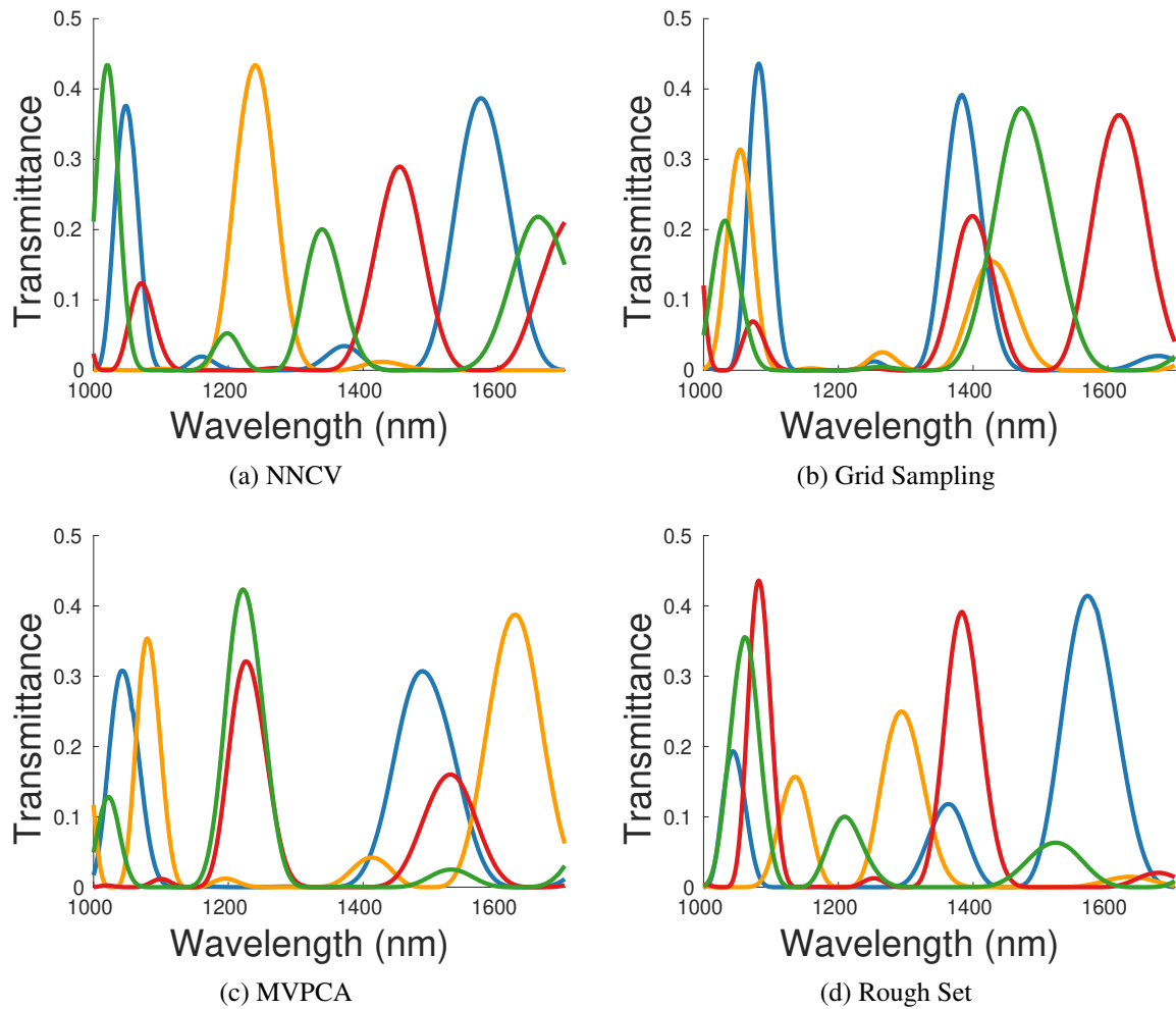
Figure 2.8: Theoretical spectral transmittance of 4 selected bands (different colors).
