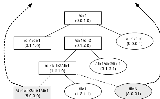
Figure 4.3: Cousin-closest OID assignment policy. The OID chosen for each element of this simple directory tree is shown. For clarity the example uses a 16 bit OID and a “.” is used to separate the value of each directory slot and file segment. The straight dashed lines show a too-deep directory overflowing to a new “root” and a file in a large directory overflowing to the too-wide region. The curved dashed lines point to the logical “parent” that the overflowed objects are assigned OIDs under.
