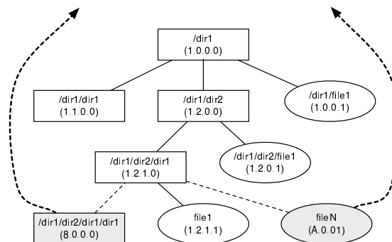
Figure 4.2: Child-closest OID assignment policy. The OID chosen for each element of this simple directory tree is shown. For clarity the example uses a 16 bit OID and a “.” is used to separate the value of each directory slot and file segment. The straight dashed lines show a too-deep directory overflowing to a new “root” and a file in a large directory overflowing to the too-wide region. The curved dashed lines point to the logical “parent” that the overflowed objects are assigned OIDs under.
